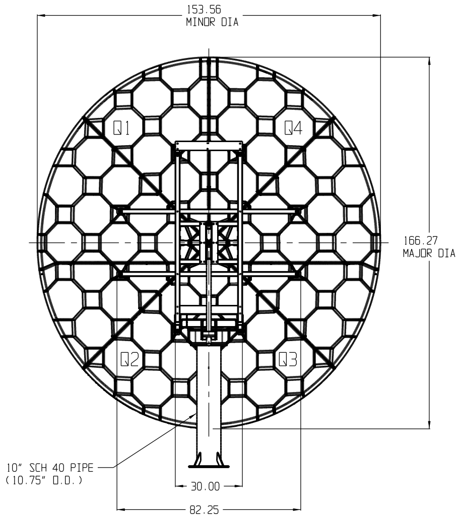
3.8M OFFSET ANTENNA GEOMETRY - 1385 SERIES
