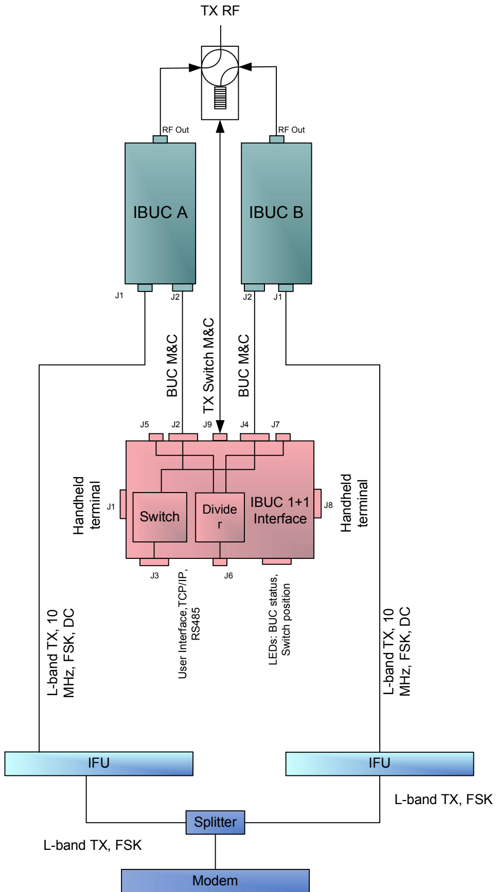
IBUC 1:1 System, TX-only IFU => DC and 10MHz
