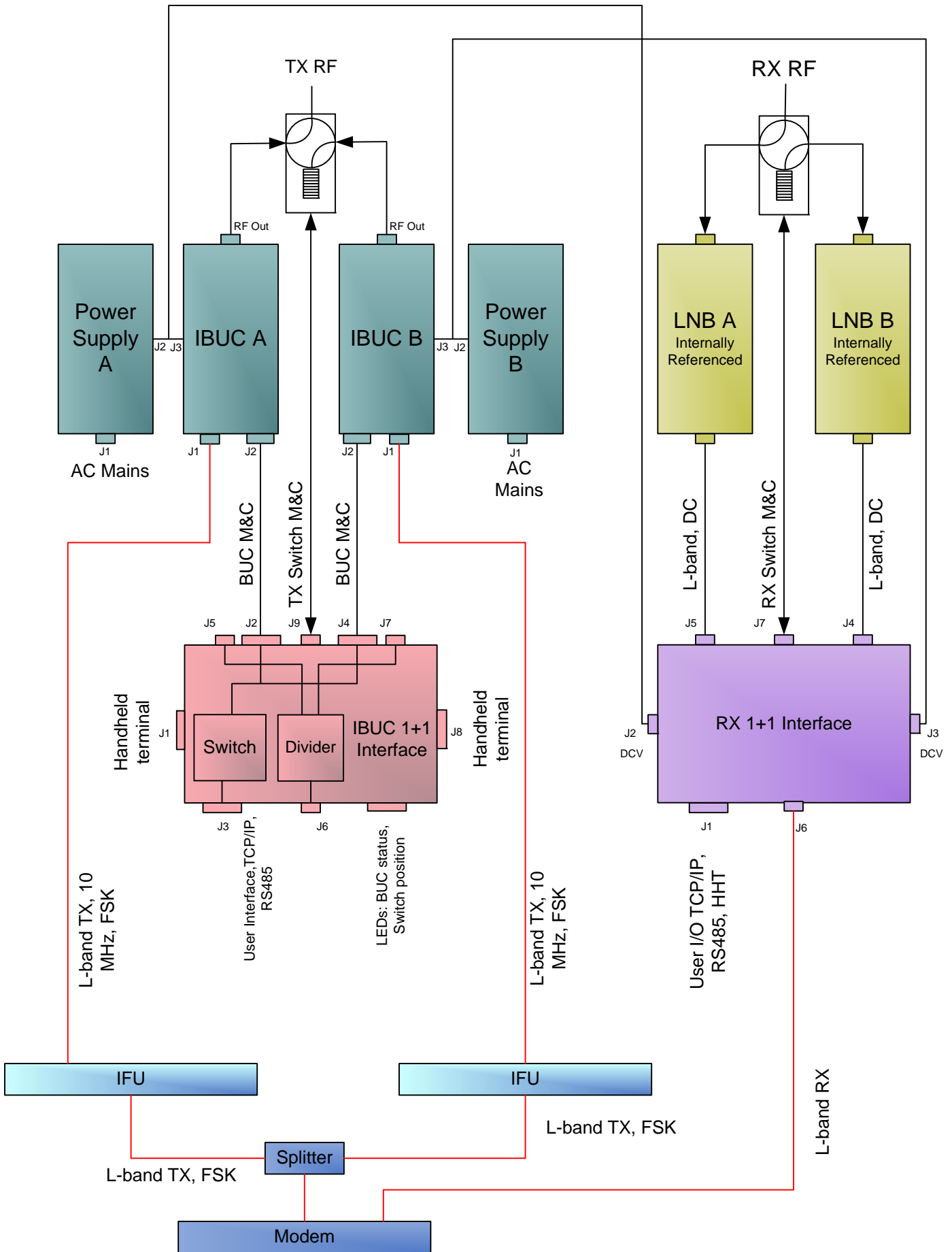
IBUC 1:1 System, Tx/RX IFU => 10MHz to BUCs LNB's => Internal reference
